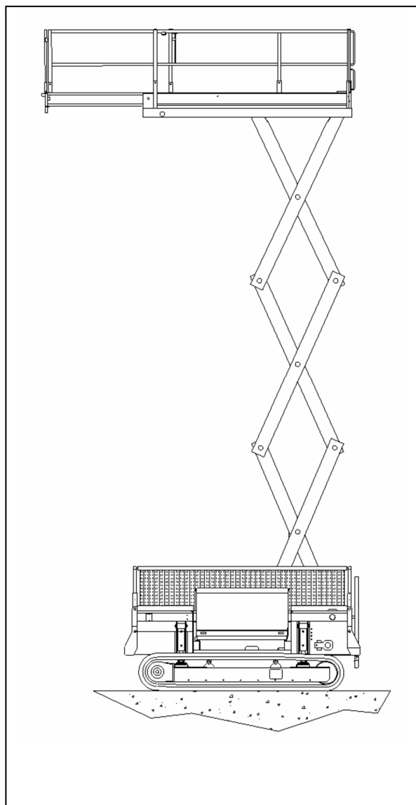
Afb. 2 Type X-Z85DL22-TR
