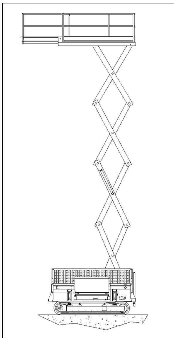
Afb. 4 Type X-105DL22-TR
