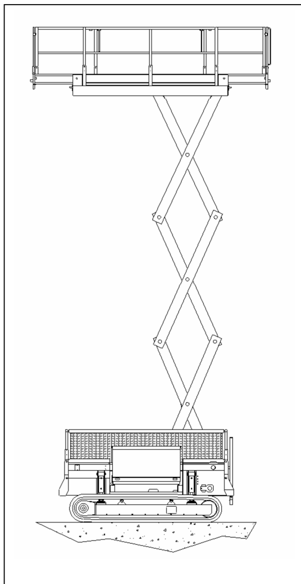
Afb. 3 Type X-Z85DXL22-TR
